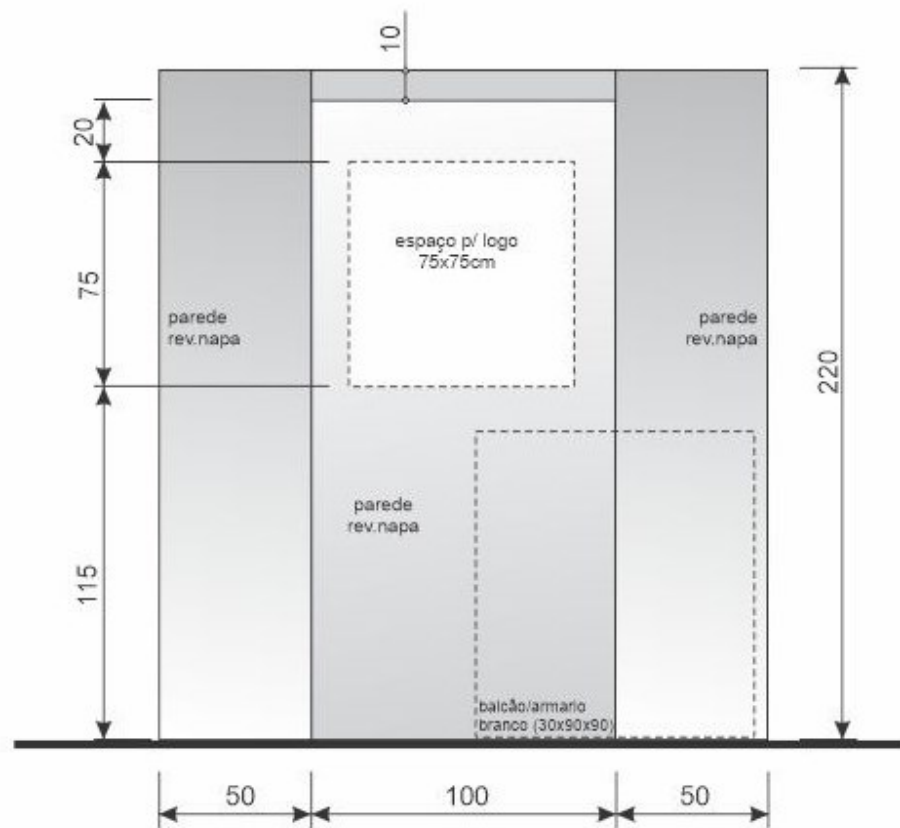
VISTA FRONTAL
